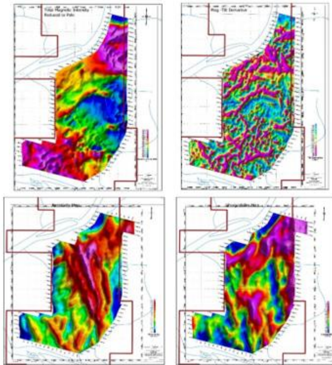
Figure 4: Sagax's elaboration: Mag and IP maps
