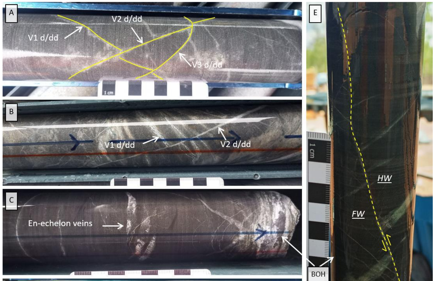
Figure 2 - Examples of mineralization and structures observed in core.
