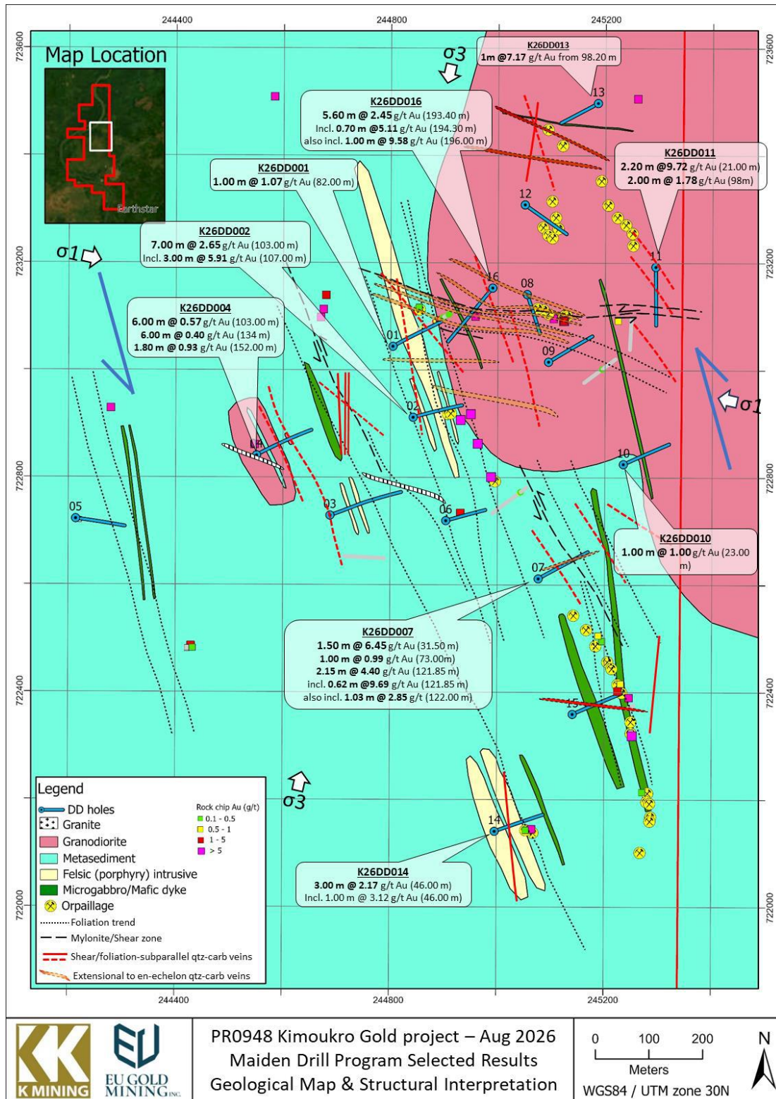
Figure 1 - Geological and structural interpretation showing the maiden diamond drill holes, principal gold intersections, interpreted mineralized vein systems and artisanal workings. Drill intervals shown are downhole lengths; true widths have not yet been established.
