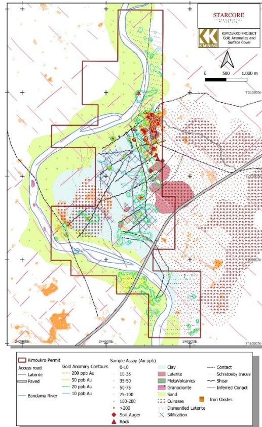
Figure 3: Distribution of gold anomaly from soil and rock samples
