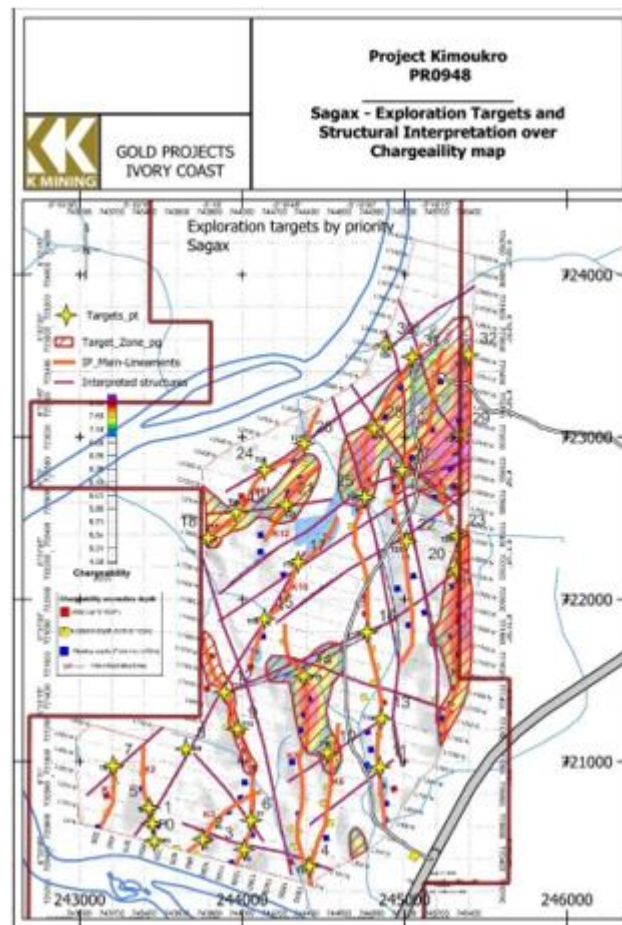
Figure 5: Map showing exploration targets proposed by Sagax over IP anomalies and structural intersections
